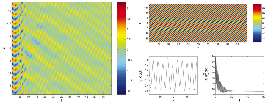
FIG. 3. (Color) The driven-damped MKdV stabilization of the breather lattice with c=1 , m=0.5 , \beta=F_0=5 . The left panel shows the space-time contour plot. The right panel top subplot shows a detail of the left plot to indicate the stabilization of the configuration. These contour plots have dimensionless units for x and t . The bottom left subplot shows the spatial profile of the solution at t=60 , while the bottom right subplot depicts the relaxational time evolution of a global property such as the discrete analog of the continuum momentum.
